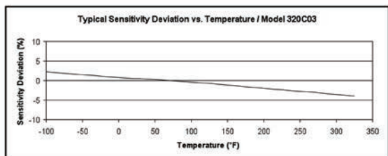
Model 320C03
