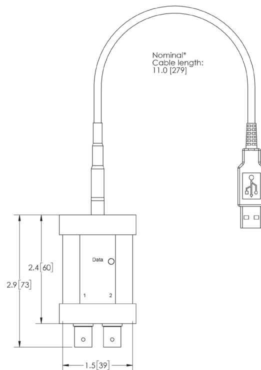
Model 485B39 Outline Drawing Dimensions in inches [mm]
